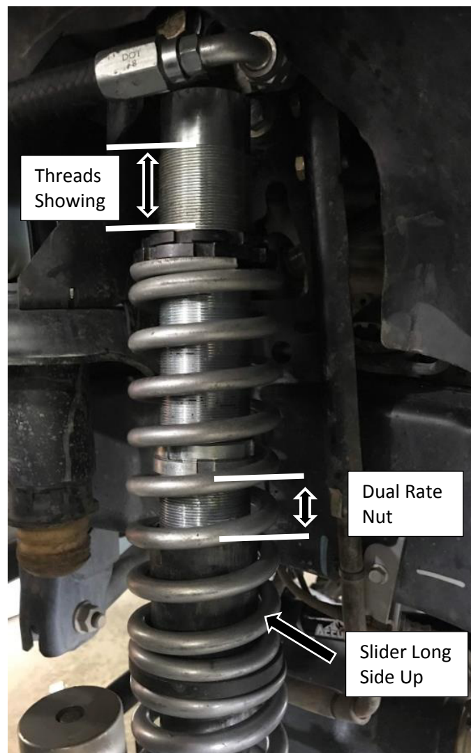
Figure 7: Coilover installation
